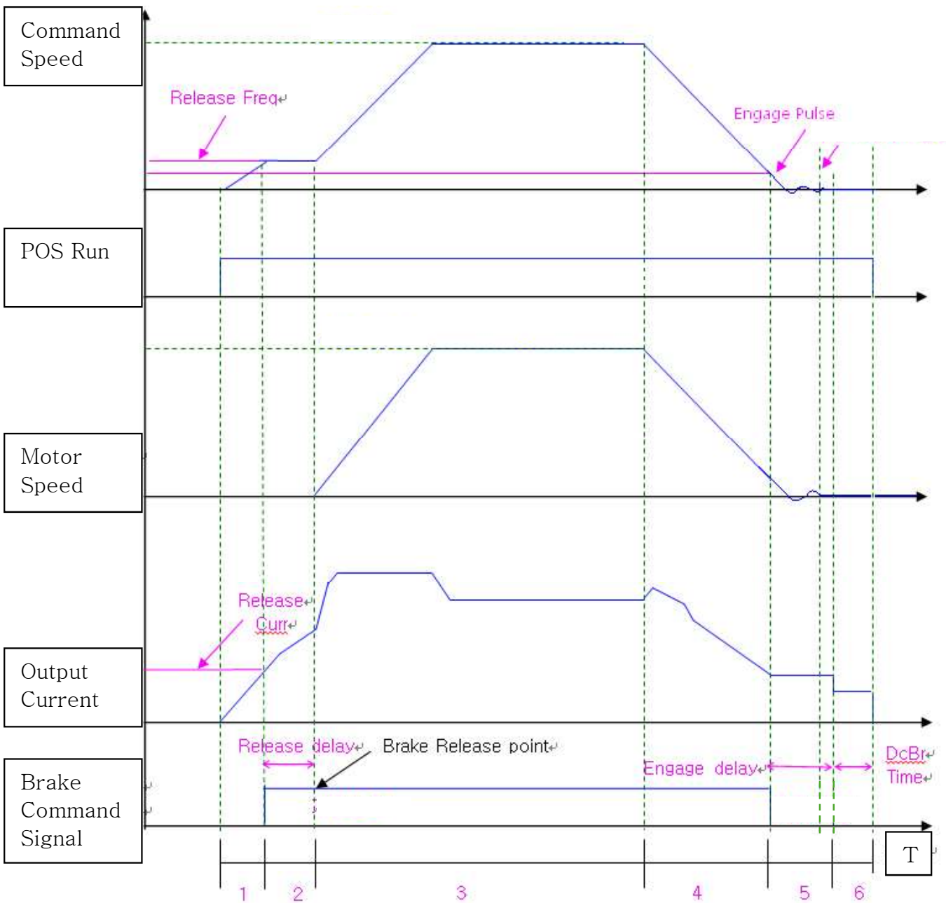
Position control with external brake operation scheme
